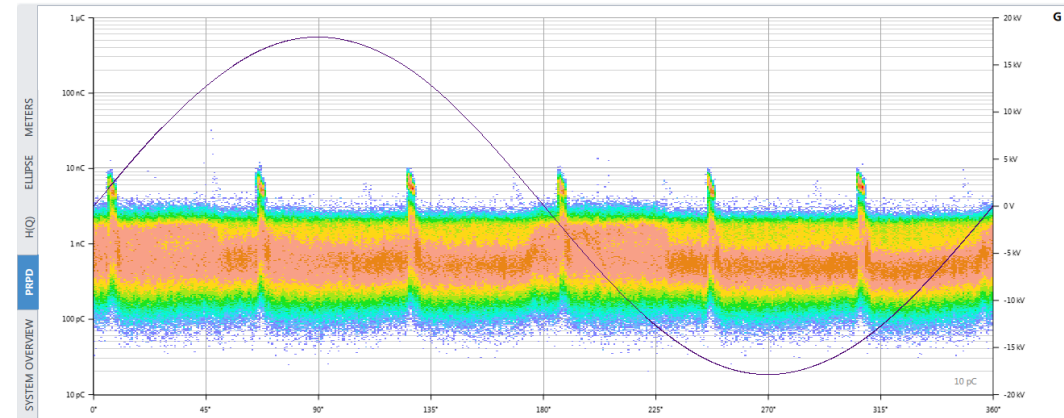
No PD detected after replacement of cable joint and cable
