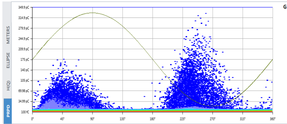
PD detected at test voltage of U_0 (12.7kV)
